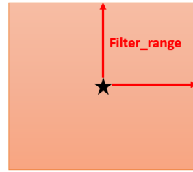
Figure 8 filter_range area.
