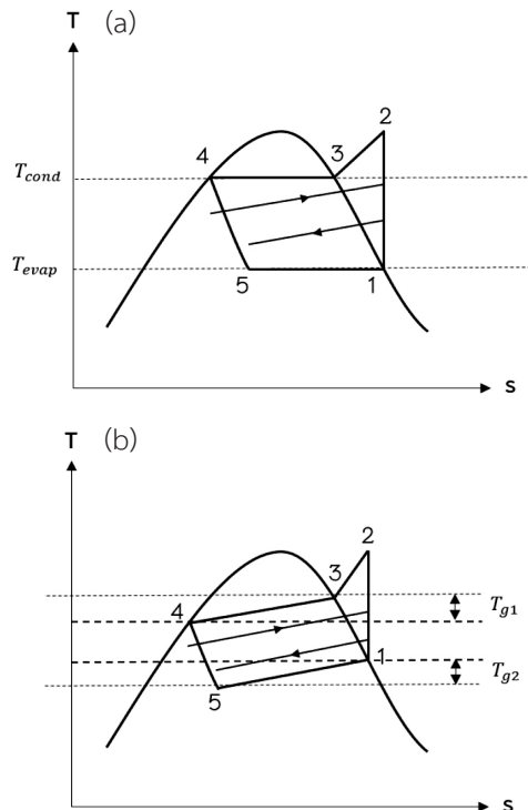
Figure 2: T-s diagram of standard heat pump cycle using (a) single refrigerant and (b) zeotropic refrigerant.
