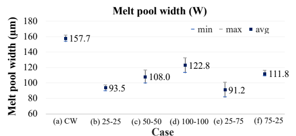
Figure 11: Comparison of the melt pool width values between all six cases.
