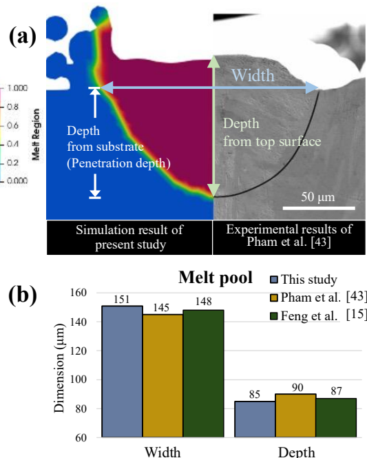
Figure 7: Comparison of the melt pool dimensions obtained in this study with the experimental results from Pham et al. , [43] and the simulation results from Feng et al. , [15]: (a) Melt pool shape and dimensions, (b) Melt pool width and depth at the top surface.
