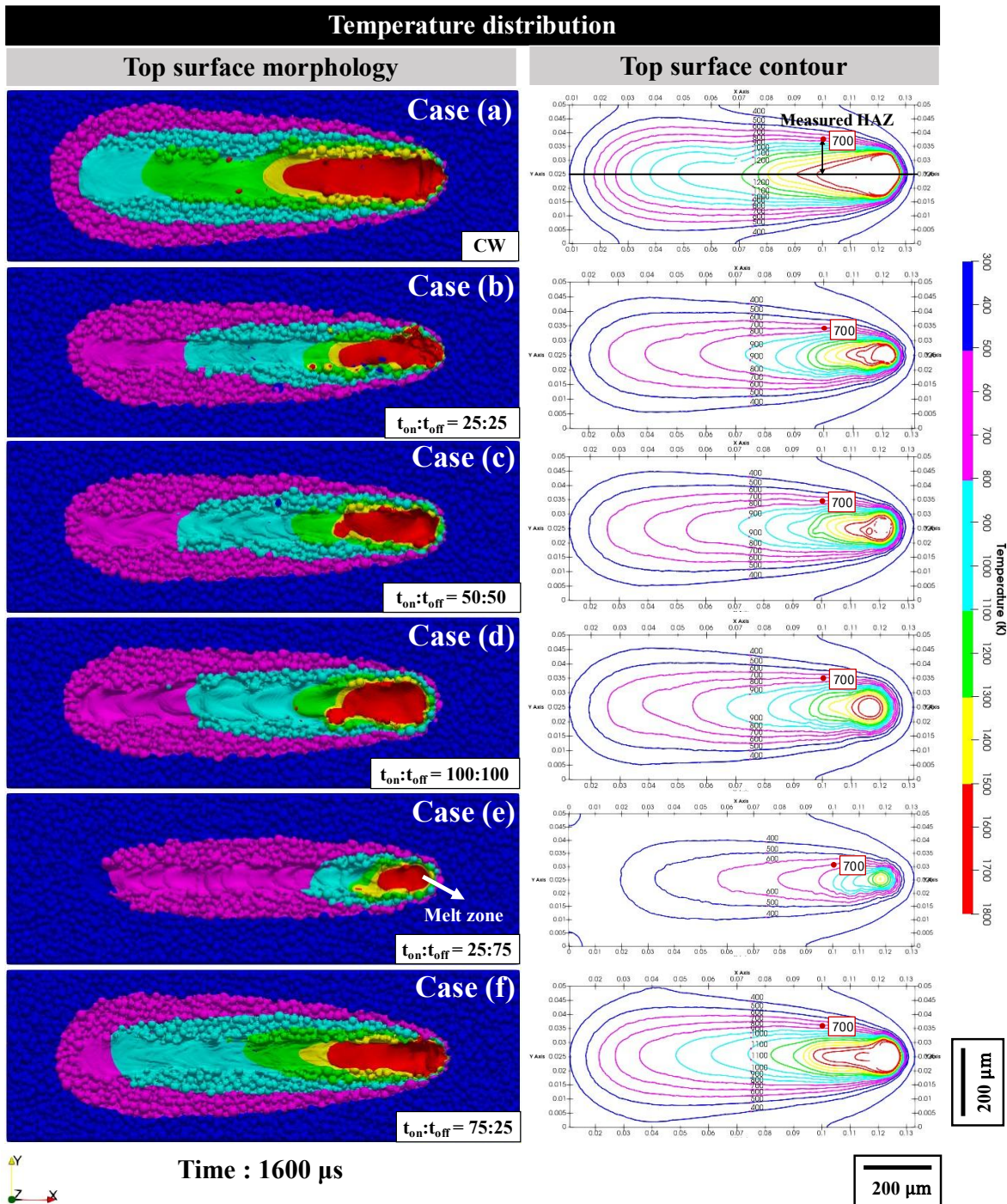
Figure 9: Melt pool shape and temperature distribution on the top surface.
