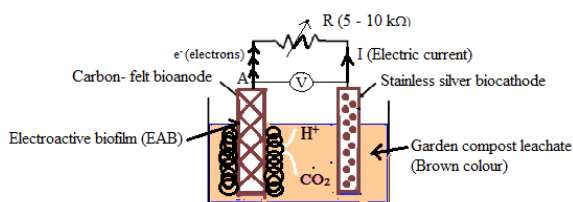
Figure 1: Schematic representation of MFCs connected to several EPRs ranging from 5–10 kΩ.
