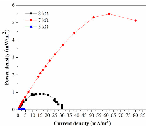
Figure 4: Power density curves of the MFCs with EPRs 5, 7, and 8 k \Omega .
