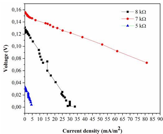
Figure 5: Polarization curves of the MFCs using EPRs 5, 7 and 8 k \Omega .
