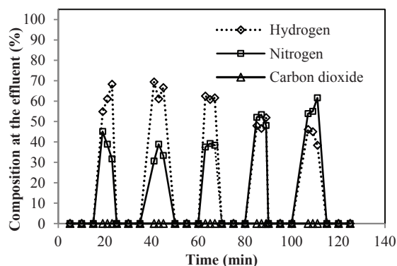
Figure 7: Dynamic adsorption separation of 50-30-20 mixture of CO 2 /H 2 /N 2 on the 0.12 wt% CHI/AC.
